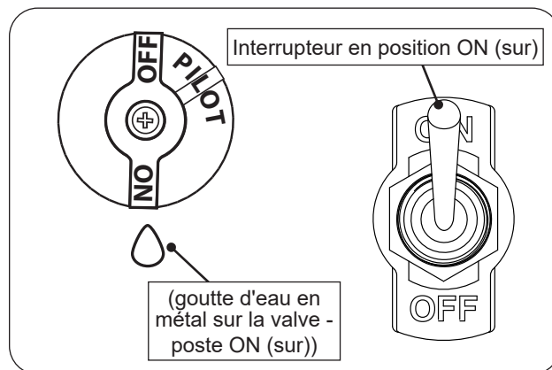
Fig. 48-1 Manual lighting
