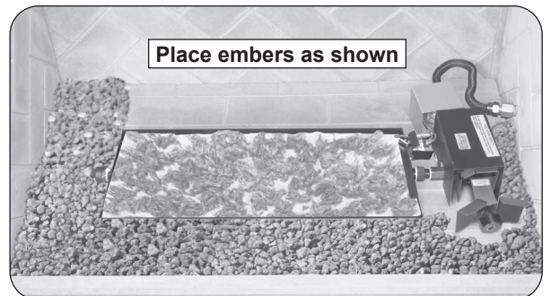
Fig. 19-3 Place glowing embers
