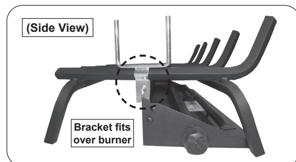
Fig. 17-3 Grate placement detail
