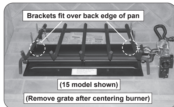
Fig. 17-2 Position grate
