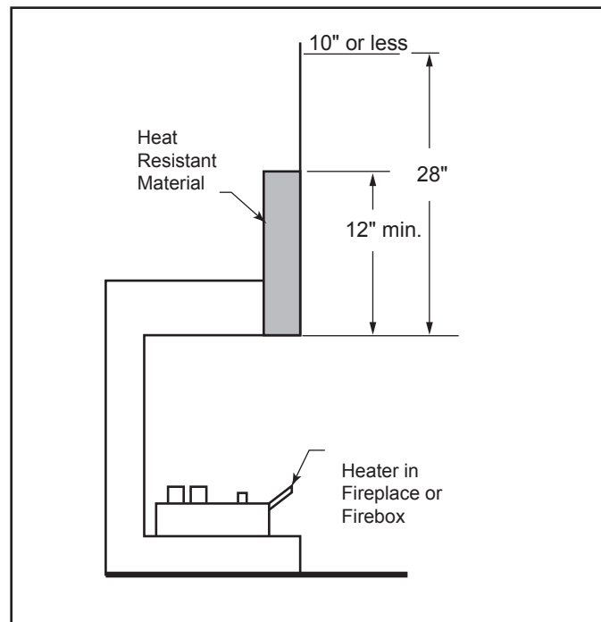
Figure 3.6 - Minimum Mantel Clearance with No Hood — MJ22/27
