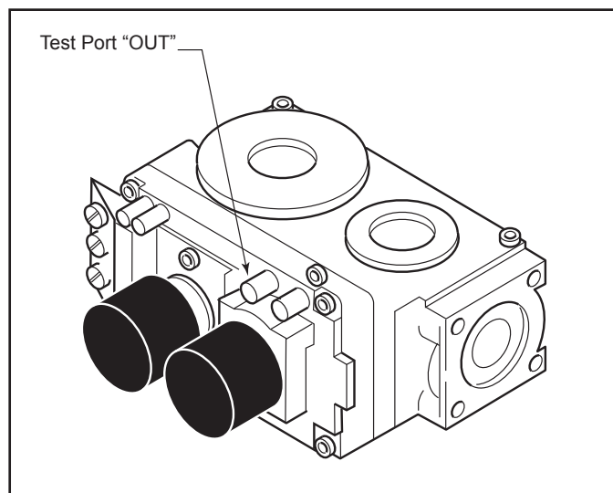
Figure 4.2 - Pressure Test Point Location Millivolt Control
