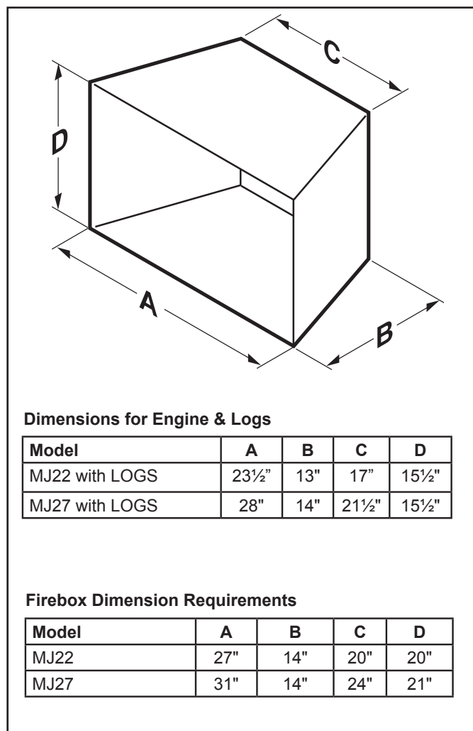
Figure 2.1 - Dimensions for Engine, Logs & Firebox
