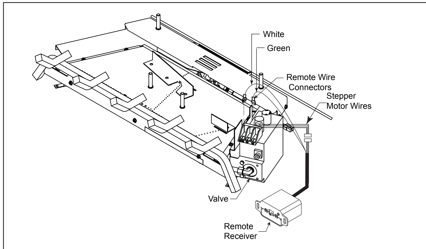
Figure 4.4 - Installing Remote Receiver
