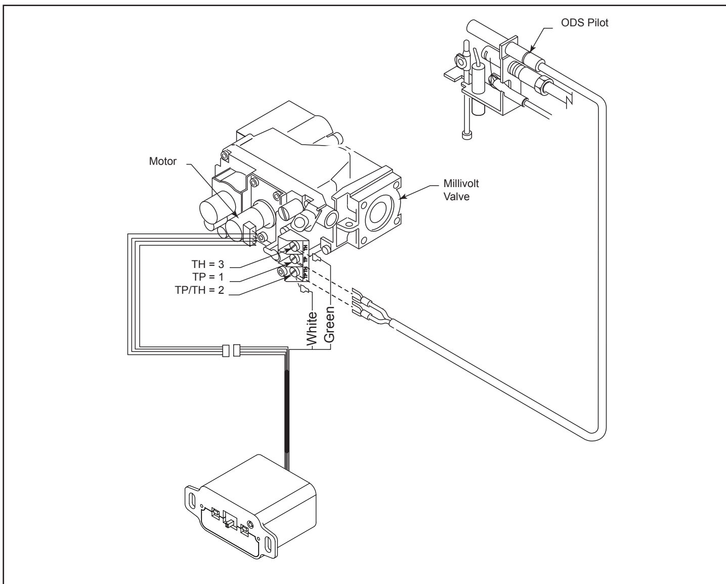
Figure 4.3 - Wiring Diagram
