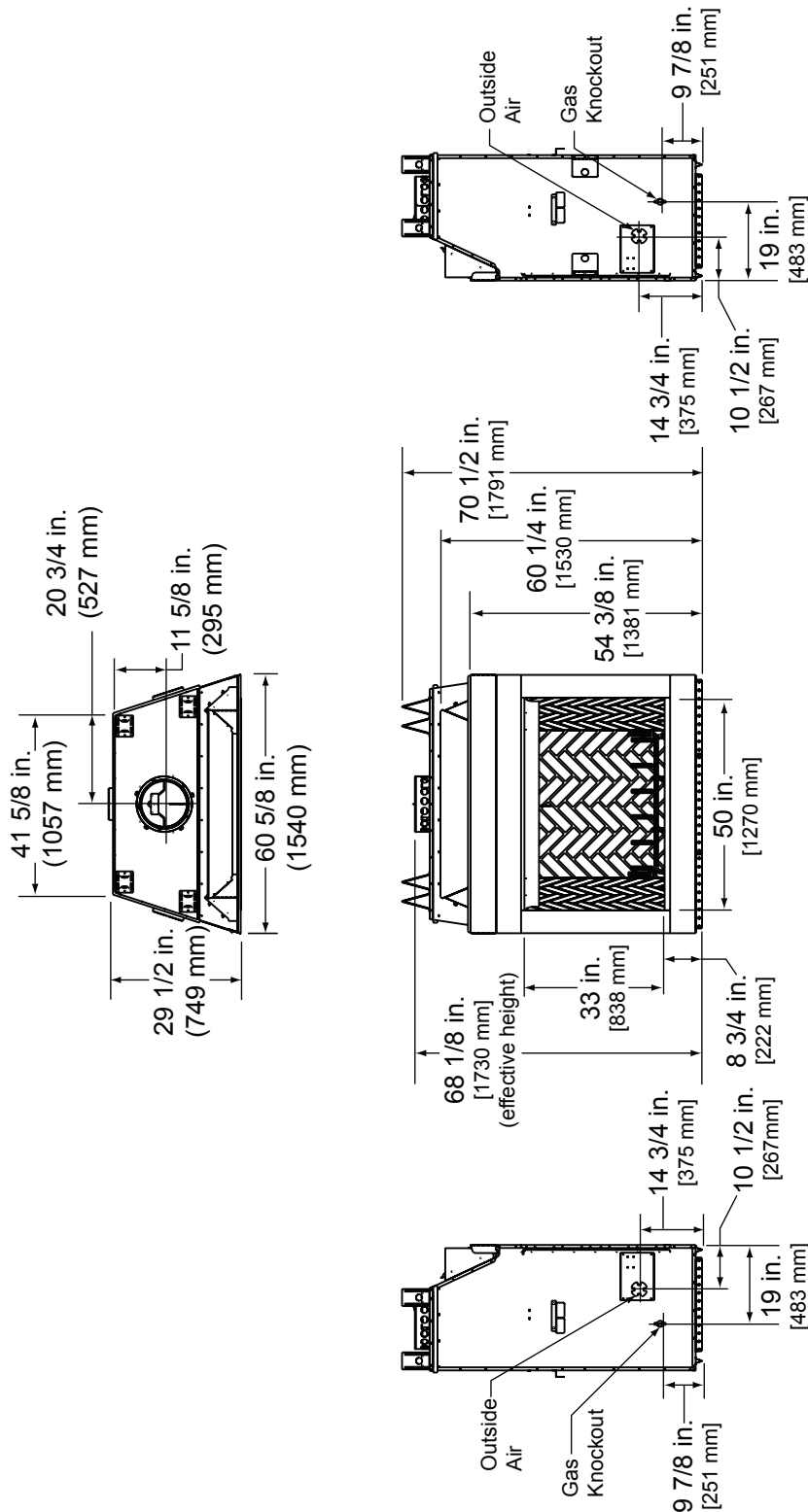
Figure 3.1 Fireplace Dimensions
