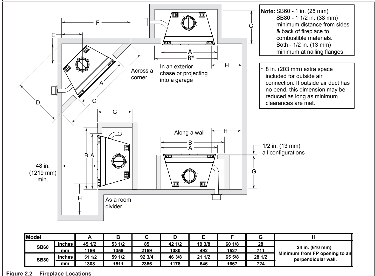
Figure 2.2 Fireplace Locations
